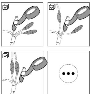
Figure 3-1 Waterproof Cables
